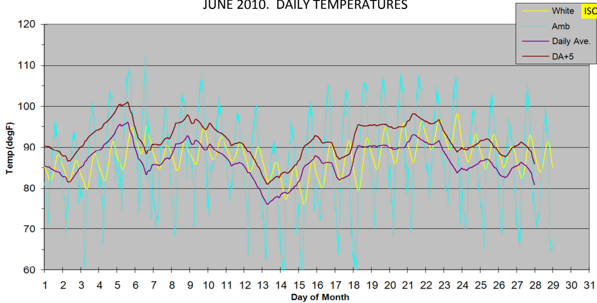
JUNE 2010. DAILY TEMPERATURES
