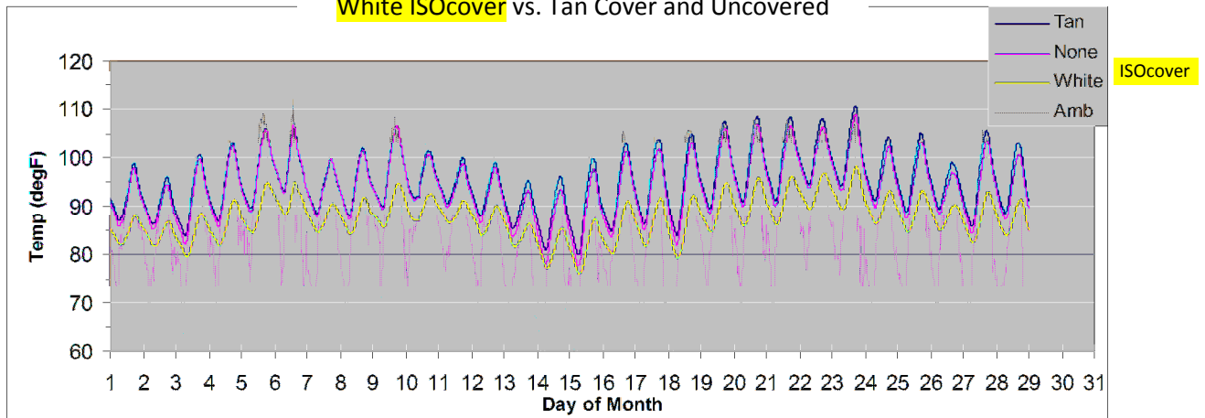
JUNE 2010. DAILY TEMPERATURES
